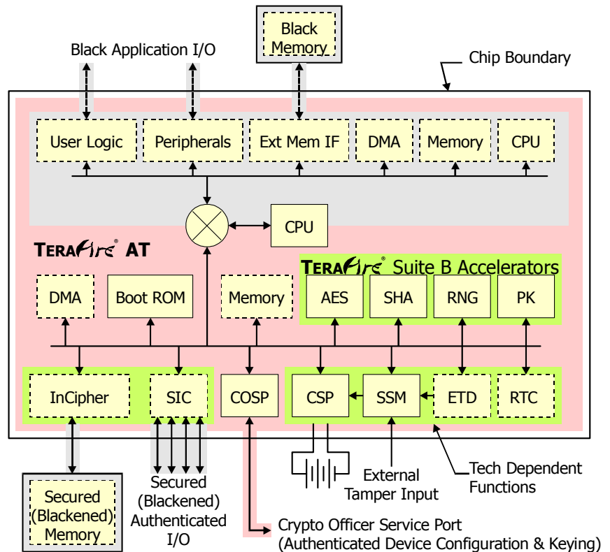
Figure 1: Example TeraFire AT-Enabled SoC
